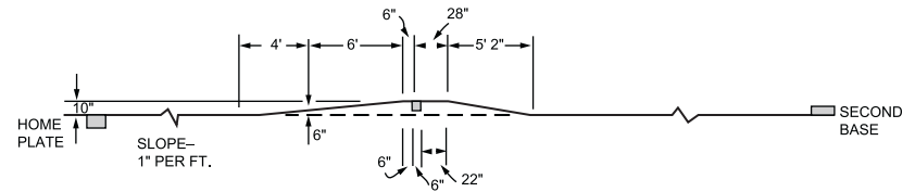
CROSS SECTION AT THE MOUND
